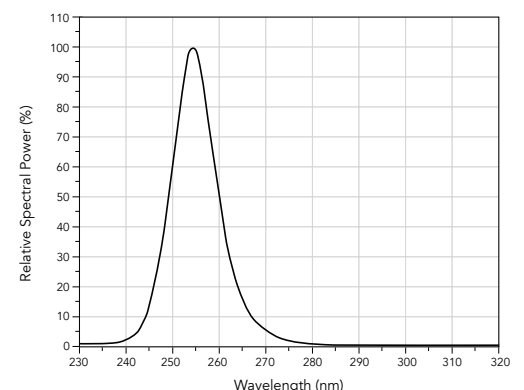
CAPL Series UVC LED Spectrum
