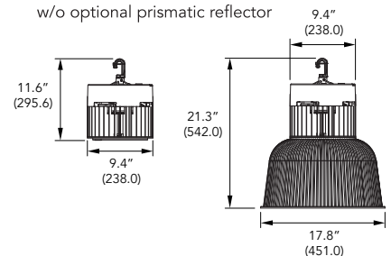
*base luminaire shown w/o optional prismatic reflector
